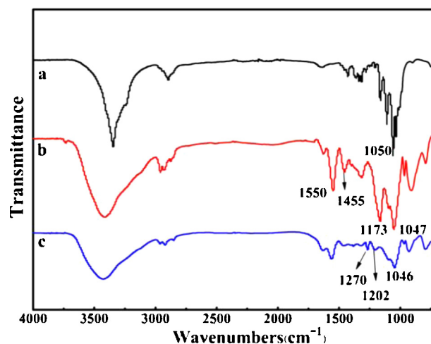
Fig. 5. FTIR spectra of pure BC (a), PPY/BC4 (b) and SPPy/BC4 (c).
